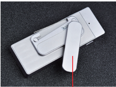
MAGNET MOUNTING
